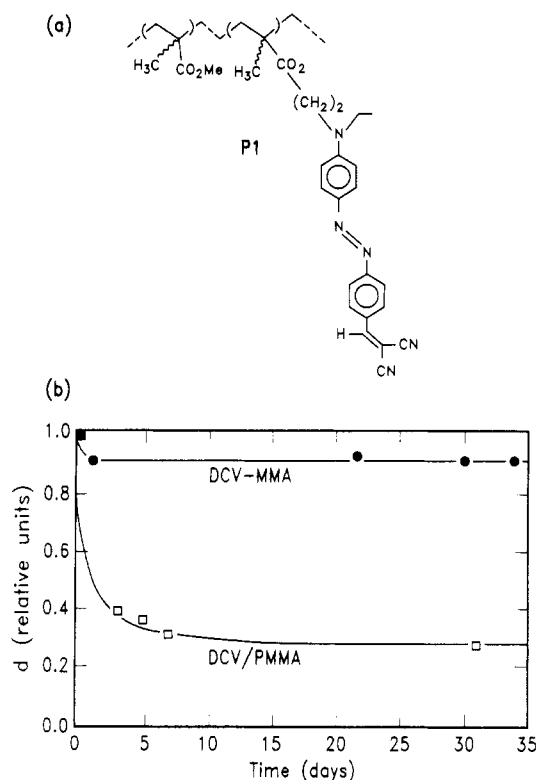
Figure 25. (a) A side-chain polymer made by random copolymerization of methyl methacrylate with a 4-(dicyanovinyl)-4'-(dialkylamino)azobenzene-substituted methacrylate (from ref 182) and (b) comparison of the decay of poled order in a film of the side-chain polymer P1 with that in a film made of PMMA doped with the same chromophore (from ref 181).
