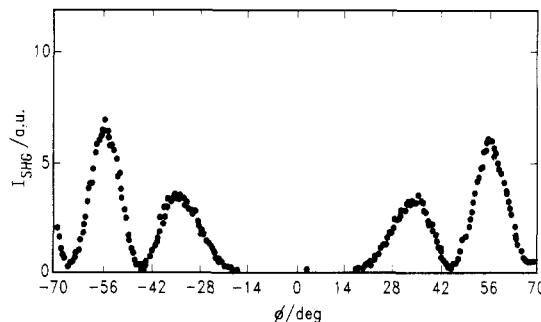
Figure 11. Typical Maker fringe curve showing SHG intensity vs \phi (defined in Figure 10) for a polymer film of thickness 94 \mu\text{m} (from ref 9).
