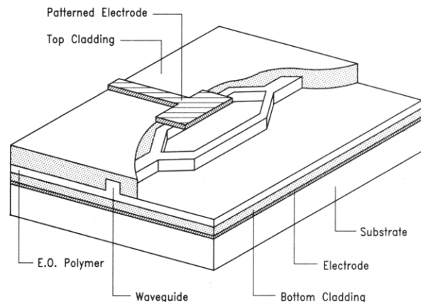
Figure 22. A waveguide Mach-Zehnder modulator (from ref 168).
